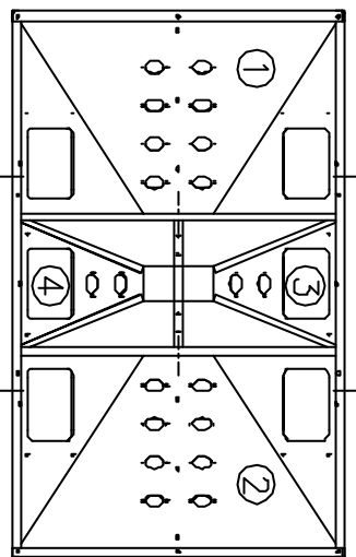
WSB 941 HOPPER-TOP VIEW
