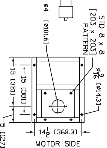
WSB-941 FOOTPRINT
